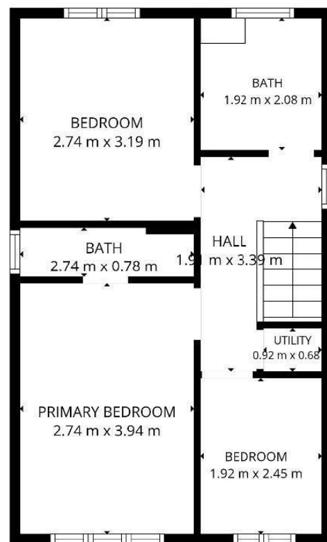
1st floor
